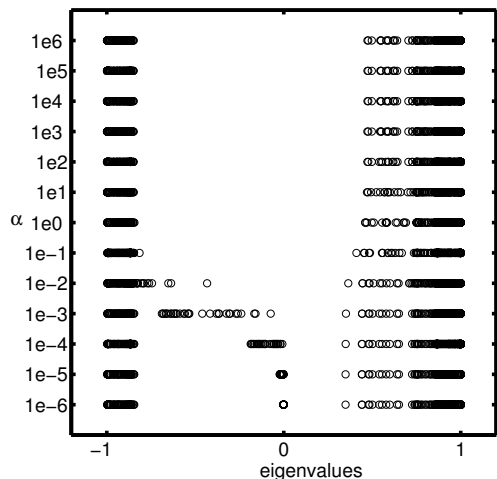
FIG. 1. Eigenvalues of preconditioned saddle point system, h = \frac{1}{16}, \alpha \in [10^{-6}, 10^6]
