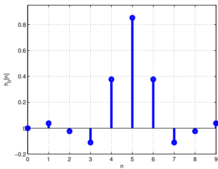
(c) Analysis low-pass filter h_0
