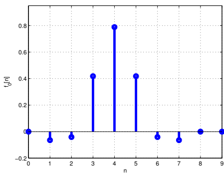
(g) Synthesis low-pass filter f_0
